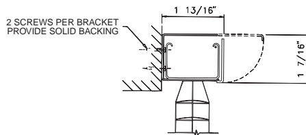
OUTSIDE MOUNTED DETAIL
