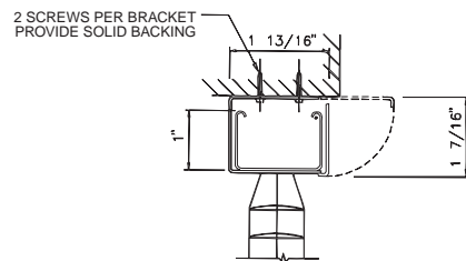
INSIDE MOUNTED DETAIL
